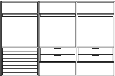
REALLY 100-9 L362,4 H240 F58
