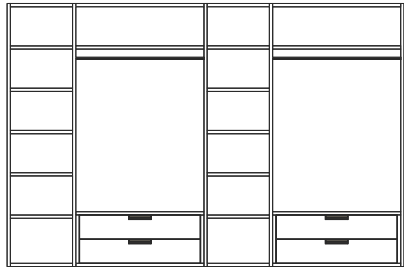
REALLY 102-6 L362,6 H240 F58
