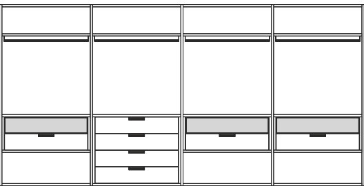
REALLY 100-1 L482,2 H240 F58
