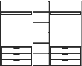
REALLY 100-7 L302,6 H240 F58
