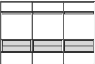
REALLY 100-3 L362,4 H240 F58
